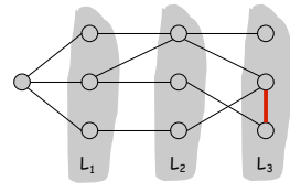
Case (ii)
