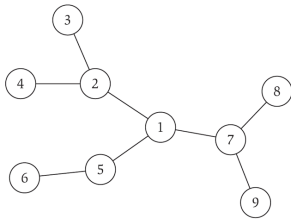
a tree
