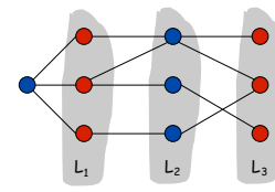
Case (i)
