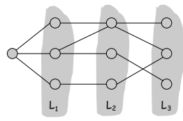
Case (i)
