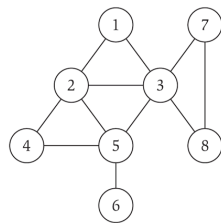
cycle C = 1-2-4-5-3-1
