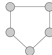
not bipartite (not 2-colorable)
