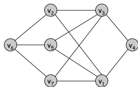
a bipartite graph G
