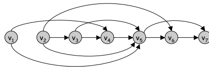
a topological ordering
