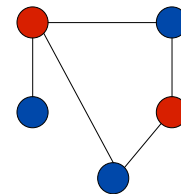
bipartite (2-colorable)
