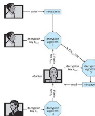
Man-in-the-middle attack - Asymmetric Cryptography
